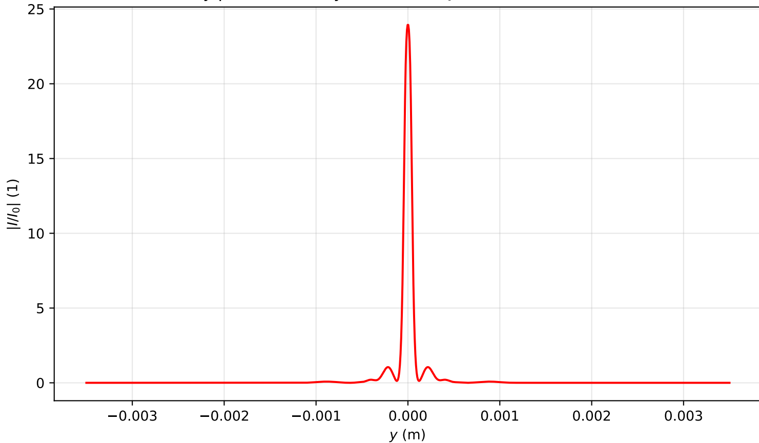
Intensity profile I(x=0, y, z=1.194)/I_0 , P_{in}=4.5P_{cr} , artificial time
